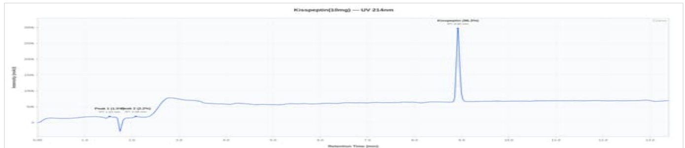
Kisspeptin 10mg - LOT-2026-001: UV Chromatogram
